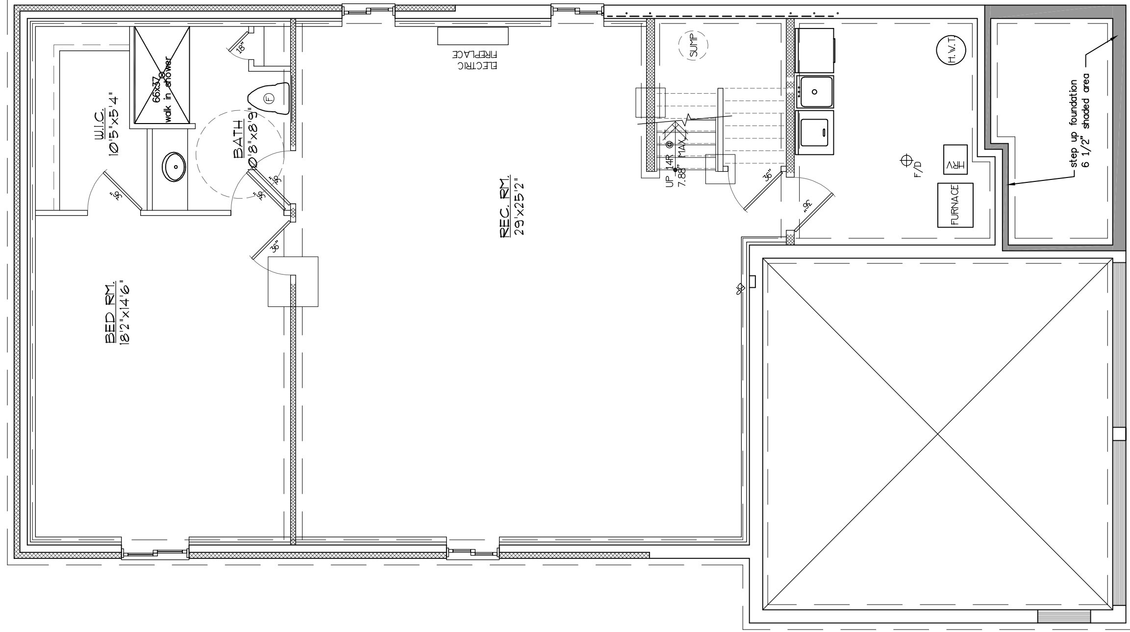
FOUNDATION PLAN FINISHED AREA = 1187 SQ. FT.
